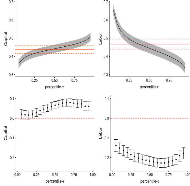
Figure 5: Estimated Coefficients of Capital and Labor for U.S. Manufacturing Firms
