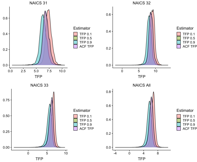
Figure 6: DS and ACF Estimates of Log Total Factor Productivity
