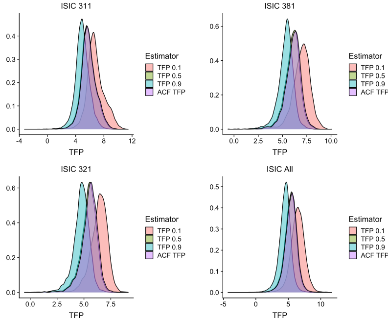
Figure 12: DS and ACF Estimates of Log Total Factor Productivity
