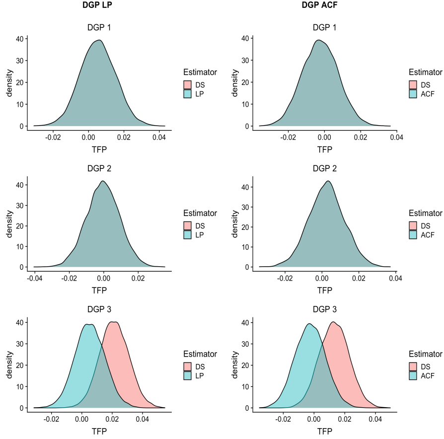
Figure 1: Monte Carlo Results for Total Factor Productivity Estimates
